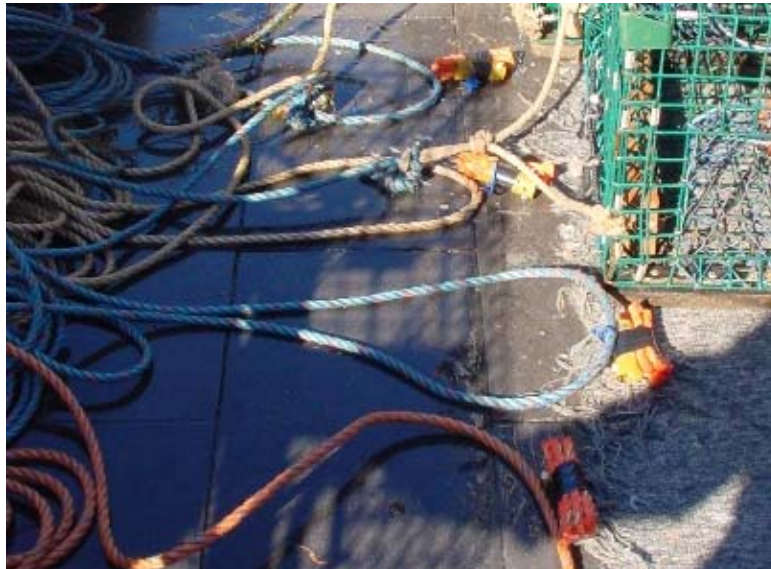
Figure 1 – pressure sensors attached to floating groundline on the boat's deck
